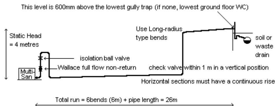
Figure 4 : Example of hydraulic selection ( equal to position B on Figure 5 )
