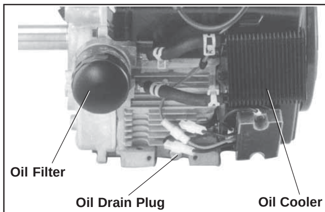
Figure 9. Oil Drain Plugs, Oil Filter, and Oil Cooler (Blower Housing Mounted).
